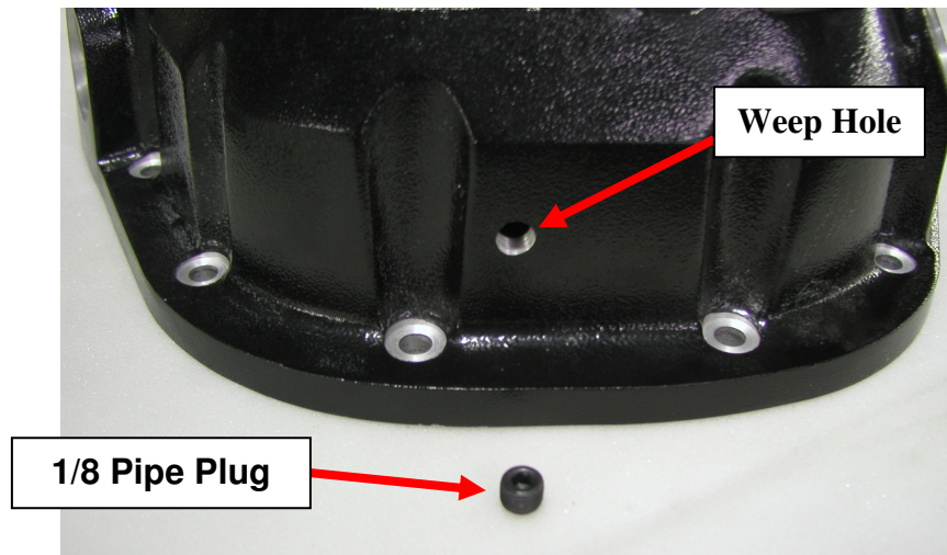
Figure 3: Weep Hole and 1/8 Pipe Plug
